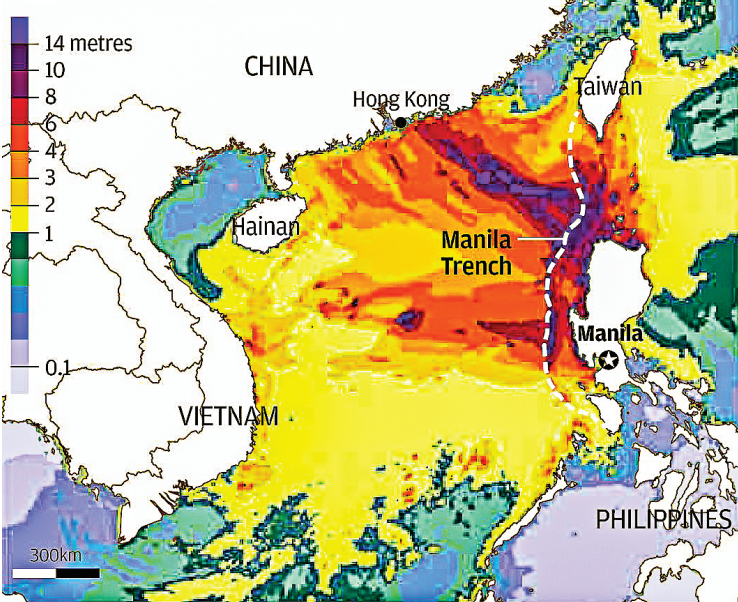
Projected wave heights within 16 hours of a magnitude-9 earthquake in the Manila Trench
